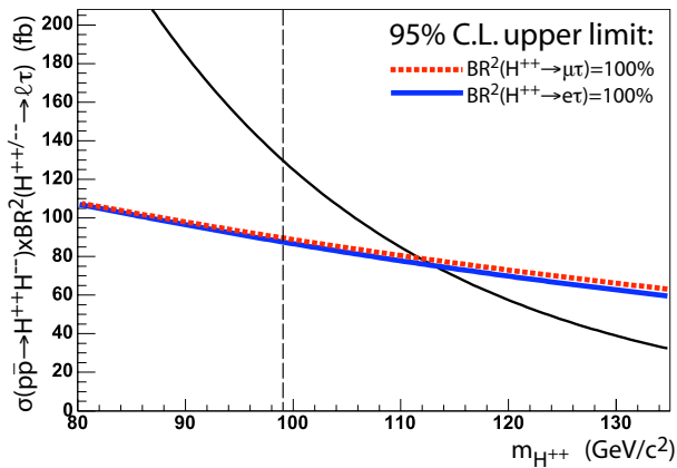
FIG. 2: Theoretical production cross sections for the pair production of left-handed H^{\pm\pm} , and 95% C.L. limit curves for \sigma(p\bar{p} \rightarrow H^{++}H^{--} \rightarrow) \times B^2(\ell^+\tau^+\ell^-\tau^-) , for \ell = e (solid), \mu (dashed). The vertical dashed line corresponds to limits from experiments at LEP2 for exclusive H_L^{\pm\pm} decays to any one dilepton channel [11].
