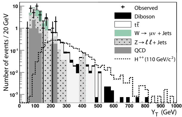
FIG. 1: The Y_T distribution in a “3- \ell ” control sample of the \mu\tau analysis that results from the application of all selection requirements except track isolation and Z removal. The signal and all backgrounds but QCD are simulated. To remain blind to the signal, Only the data points in the region Y_T < 150 GeV are inspected before unblinding the analysis.
